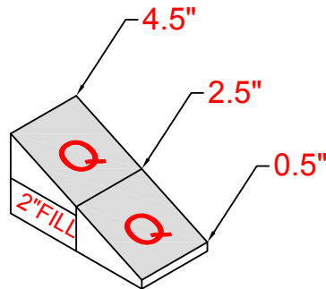
TYPICAL SECTION 1/2"/FT. SLOPE N.T.S.
